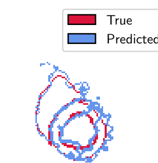
segmentations
